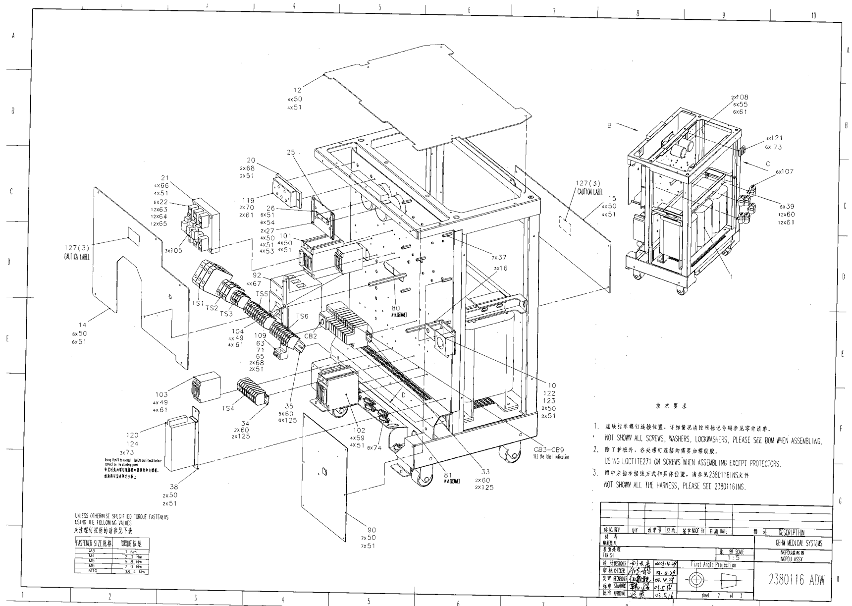
Figure 3-5 NGPDU ASSEMBLY3 (2380116, sheet 2, rev0)
