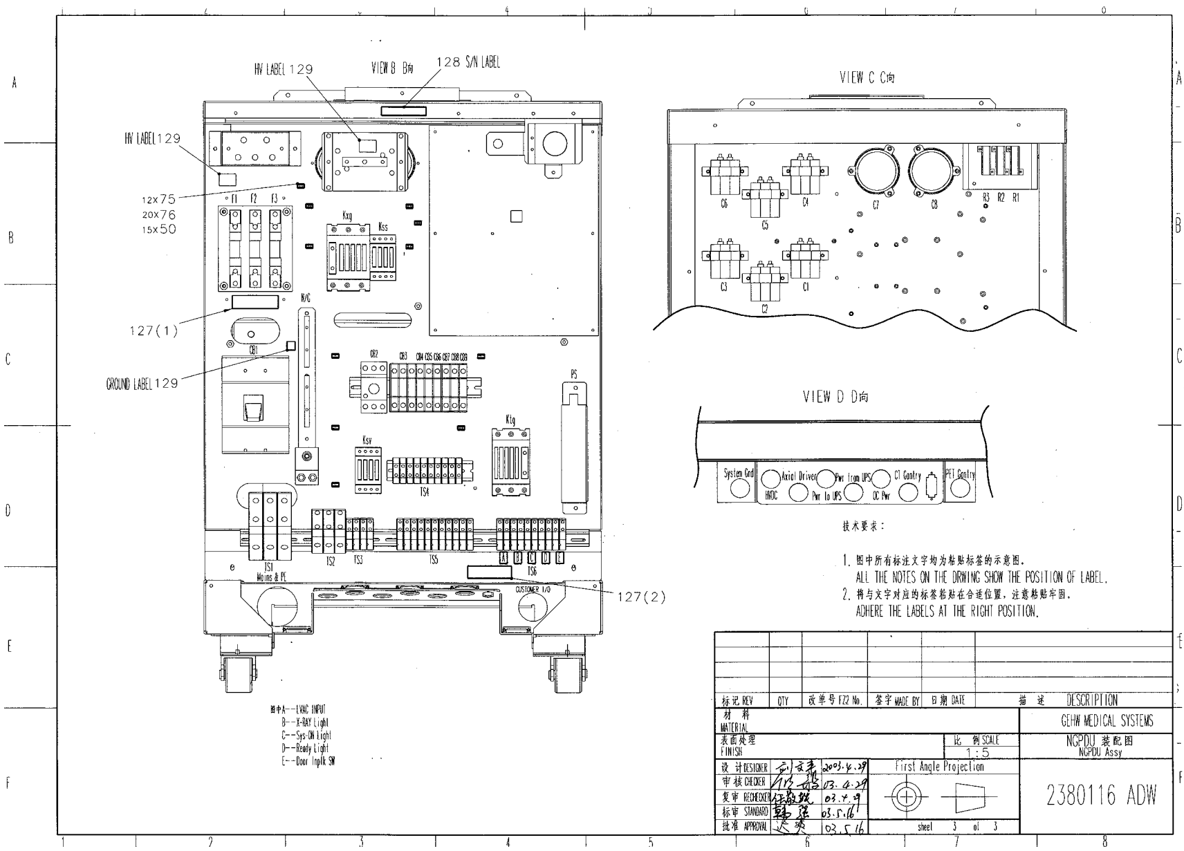
Figure 3-6 NGPDU ASSEMBLY3 (2380116, sheet 3, rev 0)
