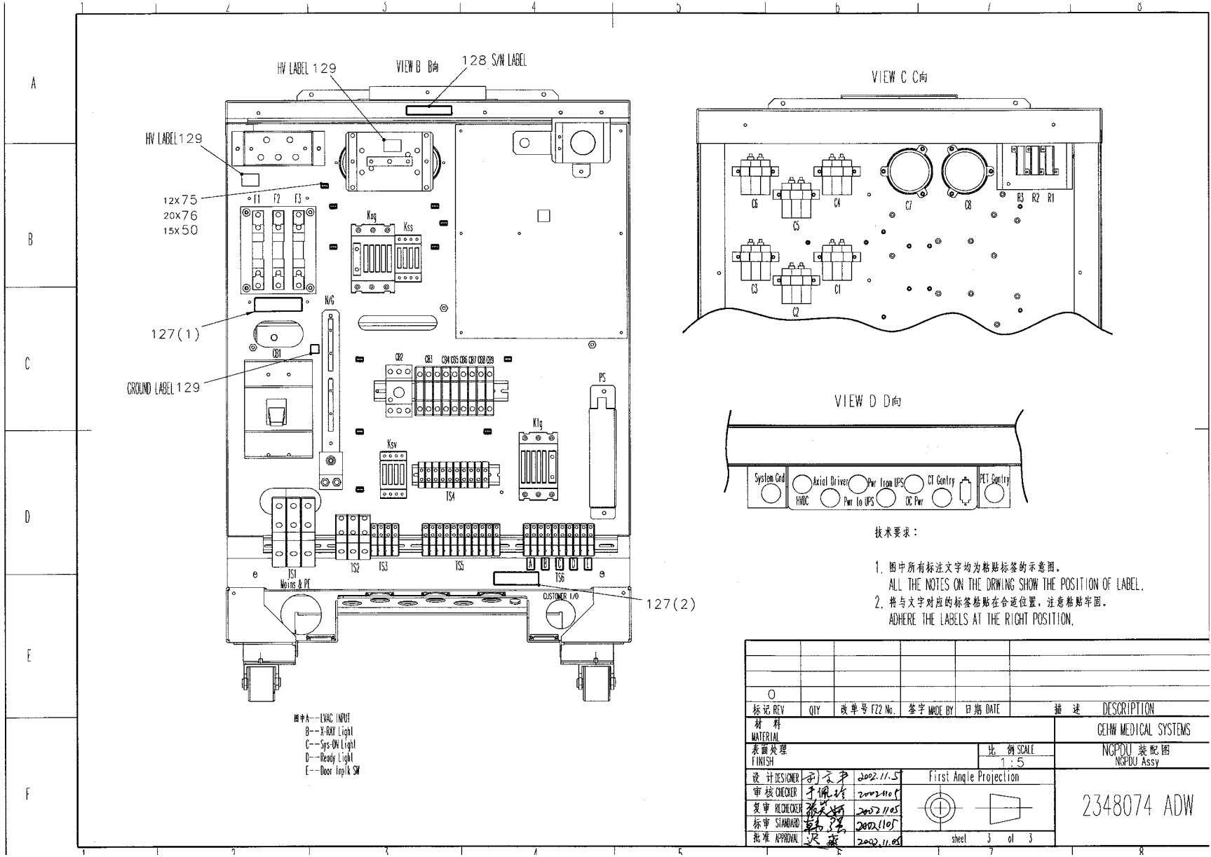
Figure 3-3 NGPDU ASSEMBLY1 (2348074, sheet 3, rev 0)
