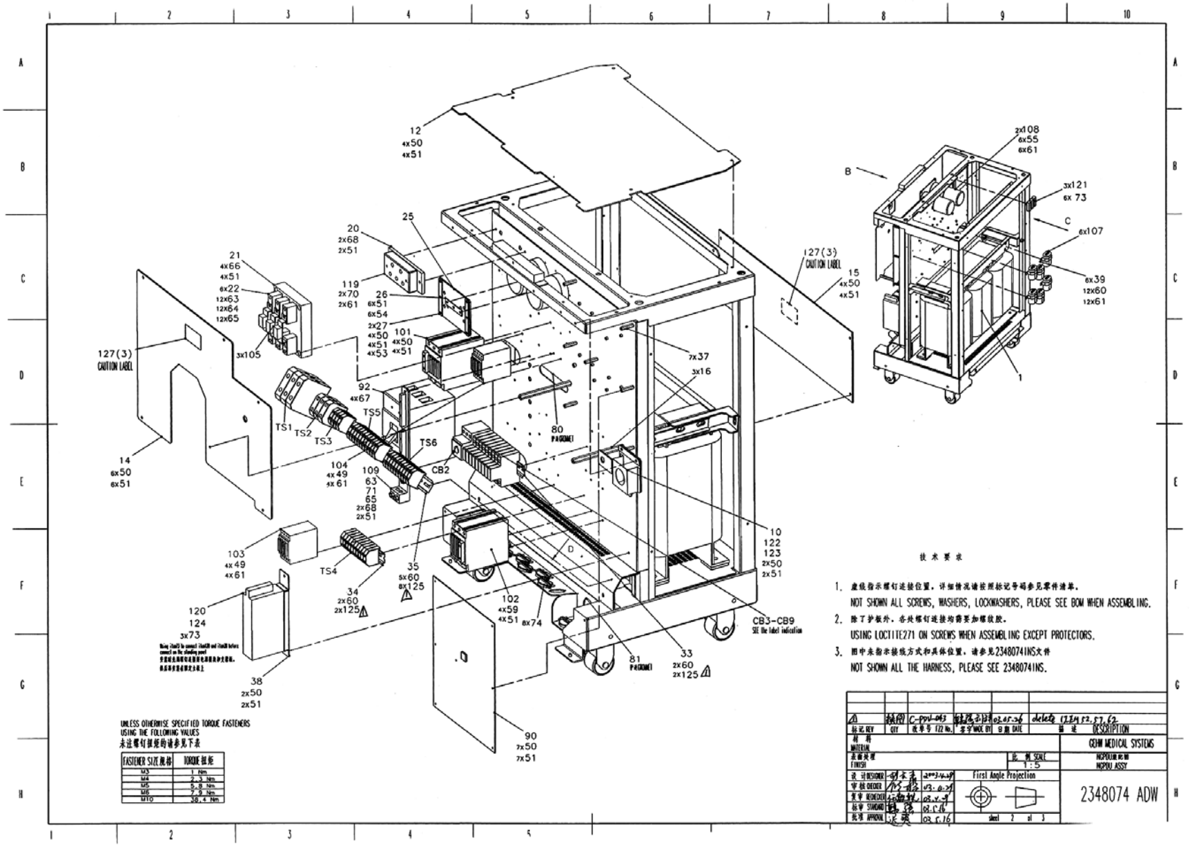
Figure 3-2 NGPDU ASSEMBLY1 (2348074, sheet 2, rev 1)
